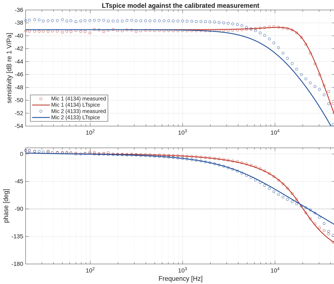
Figure 6: LTspice output (lines) against the calibrated measurement (circles), in absolute sensitivity. The LTspice source is entered with 180^\circ phase, so no extra phase shift is needed.
