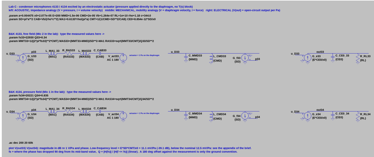
Figure 5: LTspice schematic LabC_CondenserMics.asc (rendered preview).
